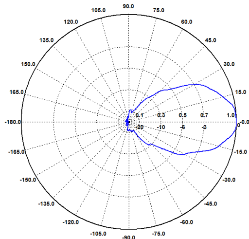
H-Ebene / H-Plane 1200 MHz
