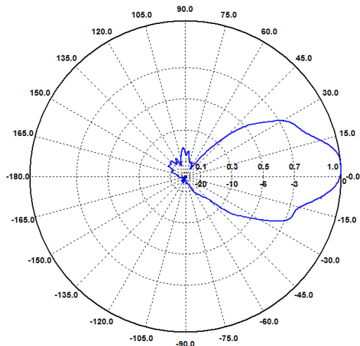
E-Ebene / E-Plane 1200 MHz
